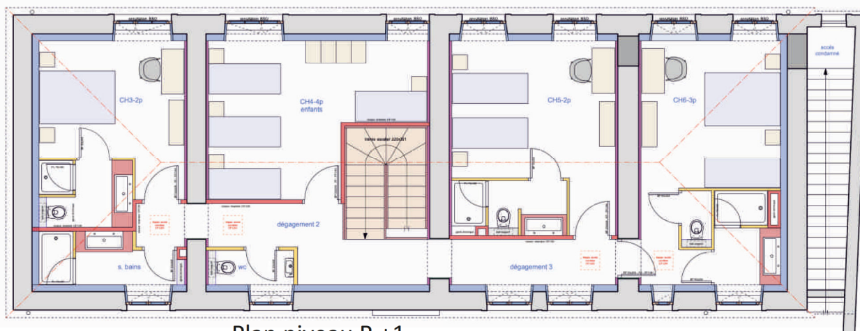
Plan niveau R +1
